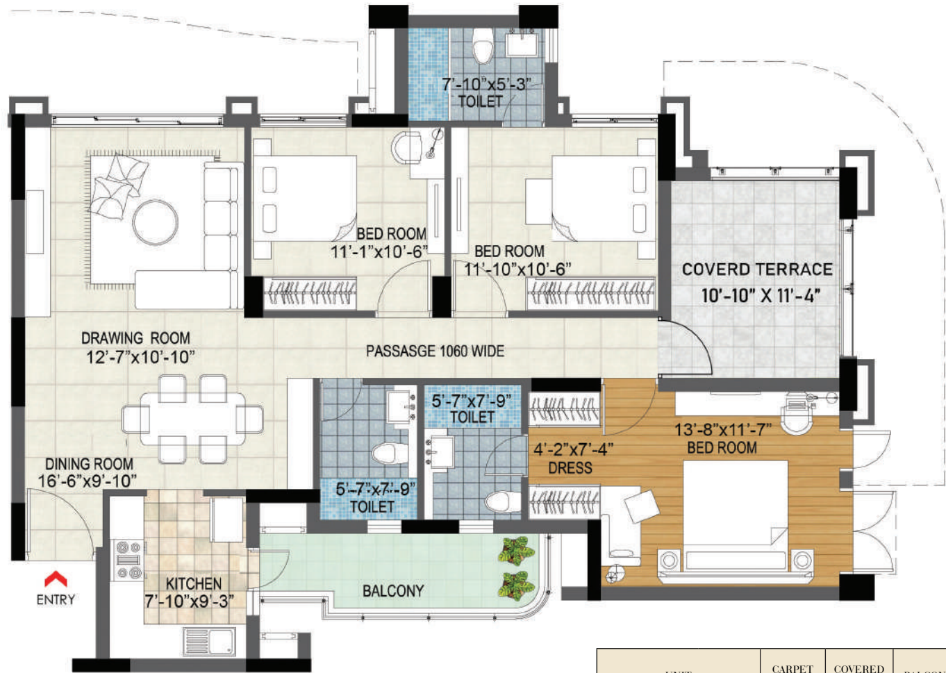
UNIT TYPE (PLAN-4) 3BHK - 1877 SQFT
