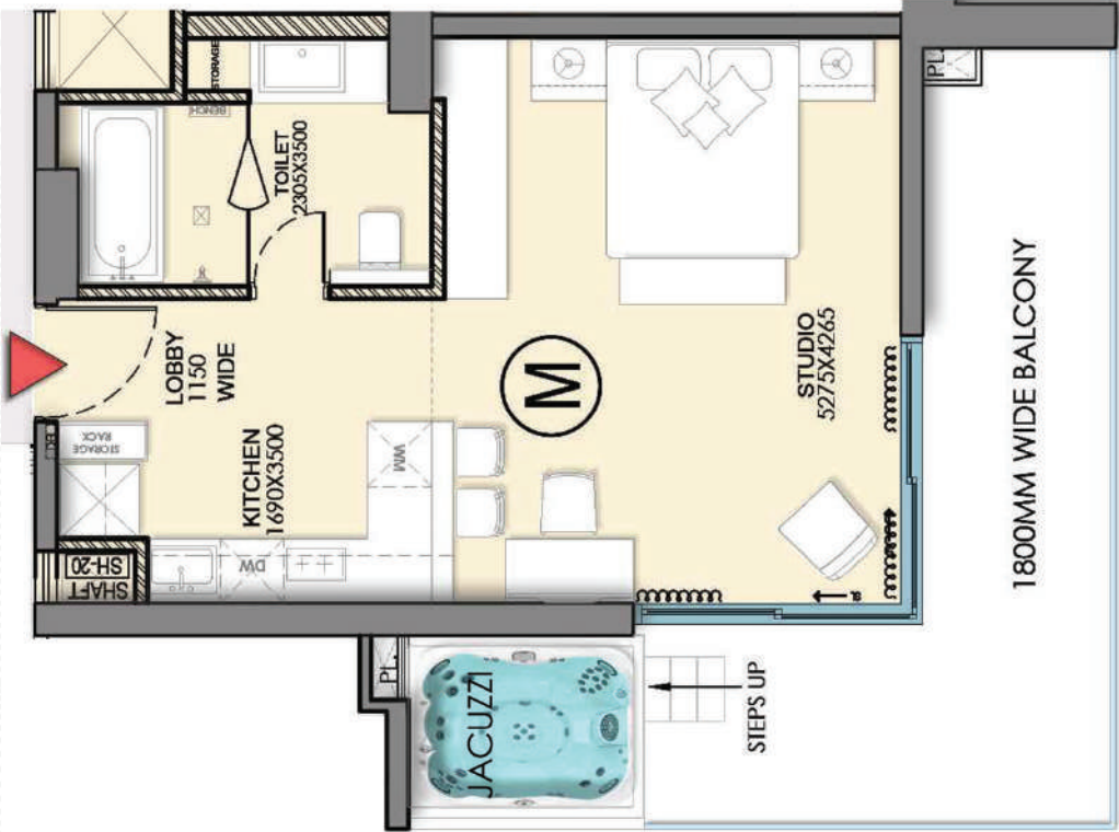
Corner Studio Residence
